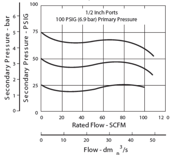
Flow Characteristics 1/2" Port
