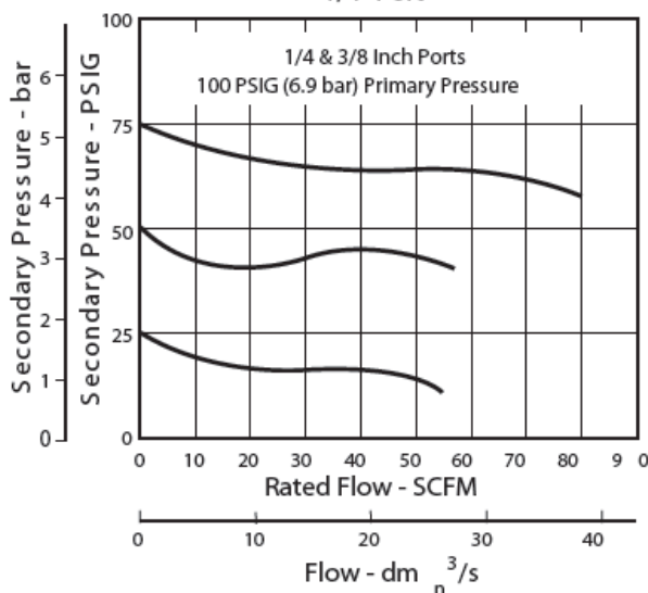
Flow Characteristics 1/4" Port
